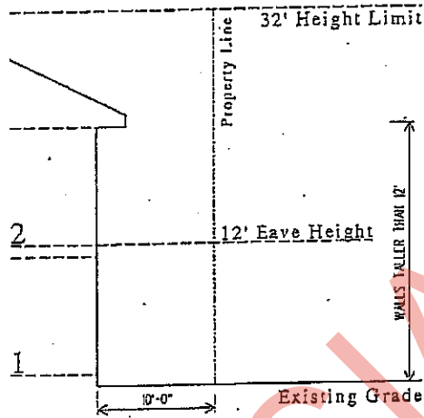
example a 2 Story Construction, 10 feet setback with walls taller than 12 feet
